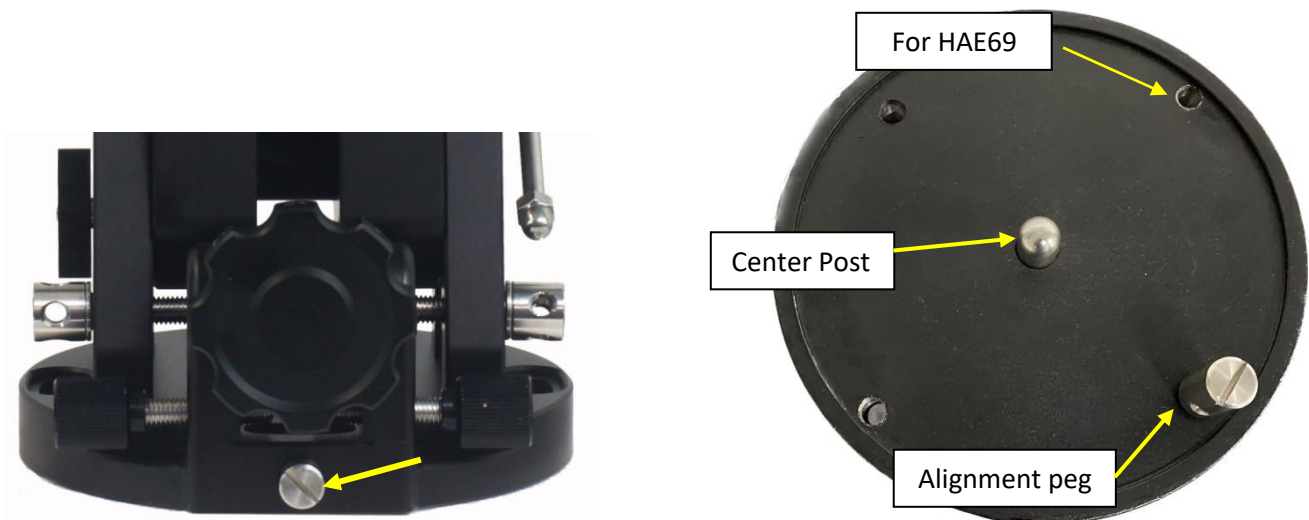
Figure 6. A LiteRoc tripod for HAE69c
